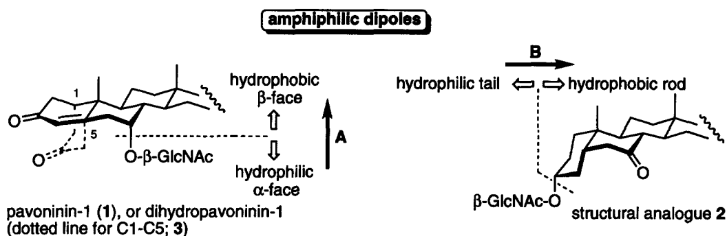
Figure 2. Amphiphilic dipoles of steroid glycosides; A: axial dipole, B; logitudinal dipole.
