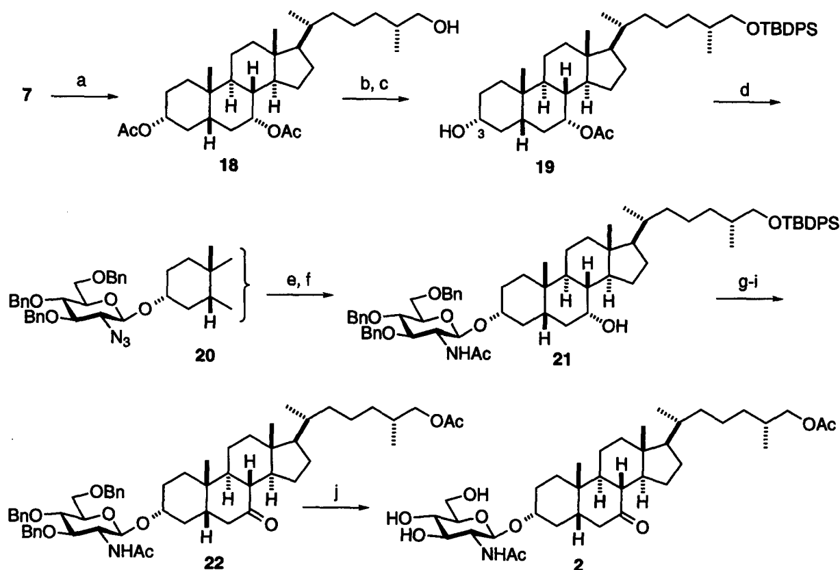
Scheme 4. Reagents and conditions: (a) \text{H}_2 , \text{Pd}(\text{OH})_2/\text{C} , \text{EtOAc-MeOH} , rt, 98%; (b) \text{TBDPSCl} , imidazole, \text{CH}_2\text{Cl}_2 , rt; (c) \text{NaOMe} , \text{MeOH} , rt, 90% (two steps); (d) 10 , \text{Tf}_2\text{O} , \text{DtBMP} , \text{CH}_2\text{Cl}_2 , -78^\circ\text{C} , then 19 , 70%; (e) \text{LiAlH}_4 , \text{THF} , rt; (f) \text{Ac}_2\text{O} , pyridine, \text{MeOH-CH}_2\text{Cl}_2 , 0^\circ\text{C} , 54% (two steps); (g) \text{PDC} , \text{MS4A} , \text{CH}_2\text{Cl}_2 , rt, 81%; (h) \text{TBAF} , \text{THF} , rt; (i) \text{Ac}_2\text{O} , \text{DMAP} (cat.), pyridine- \text{CH}_2\text{Cl}_2 , rt, 88% (two steps); (j) \text{H}_2 , \text{Pd}(\text{OH})_2/\text{C} , \text{EtOH} , rt, 87%.
