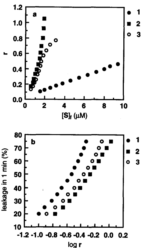
Figure 5. (a) Binding isotherms for three steroid glycosides 1 , 2 and 3 with PC liposomes. (b) Membrane permeabilizing ability of the bound glycosides.
