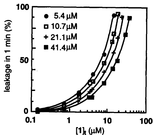
Figure 3. Dependency of calcein leakage from PC liposomes by pavoninin-1 ( 1 ) on lipid concentrations.
