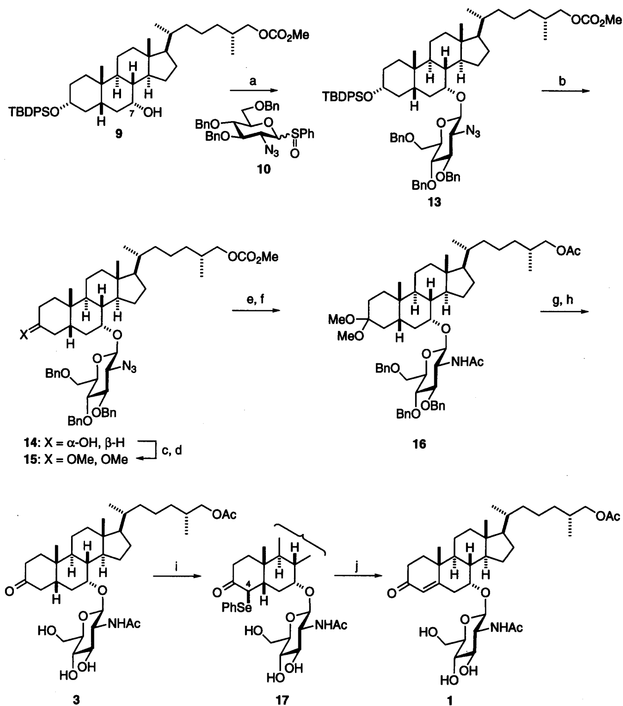
Scheme 3. Reagents and conditions: (a) 10 , \text{Ti}_2\text{O}_3 , DtBMP, \text{CH}_2\text{Cl}_2 , then 9 , -78 to -20 ^\circ\text{C} , 97%; (b) 46% HF aq, MeCN, rt, 96%; (c) PDC, MS4A, \text{CH}_2\text{Cl}_2 , rt, 95%; (d) \text{CH}(\text{OMe})_3 , CSA, MeOH, \text{CH}_2\text{Cl}_2 , rt, 96%; (e) \text{LiAlH}_4 , THF, rt; (f) \text{Ac}_2\text{O} , pyridine, DMAP (cat.), \text{CH}_2\text{Cl}_2 , rt, 89% (two steps); (g) \text{H}_2 , \text{Pd}(\text{OH})_2/\text{C} , MeOH, rt; (h) \text{AcOH} , \text{H}_2\text{O} , rt, 87% (two steps); (i) \text{PhSeCl} , EtOAc, rt, 30%; (j) 30% \text{H}_2\text{O}_2 , THF, 0 ^\circ\text{C} , 82%.
