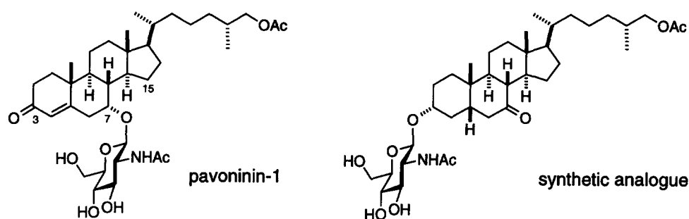
Figure 1. Structure of pavoninin-1 (1) and its synthetic analogue (2).
