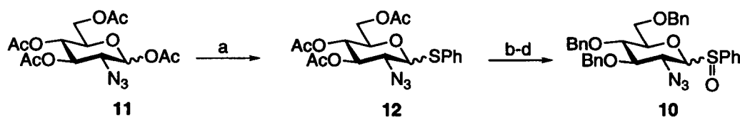
Scheme 2. Reagents and conditions: (a) PhSH, \text{BF}_3 \cdot \text{OEt}_2 , \text{CH}_2\text{Cl}_2 , reflux, 77%; (b) NaOMe, MeOH, rt, 94%; (c) NaH, BnBr, TBAI, DMF, rt, 89%; (d) m CPBA, \text{CH}_2\text{Cl}_2 , -78 to 0^\circ\text{C} , 83%.
