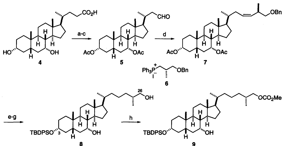
Scheme 1. Reagents and conditions: (a) \text{Ac}_2\text{O} , pyridine, DMAP (cat.), 88%; (b) \text{Pb}(\text{OAc})_4 , \text{I}_2 , hv, \text{CCl}_4 , reflux, 70%; (c) DMSO, 2,4,6-collidine, 150 °C, 90%; (d) 6 , NaHMDS, 0 °C to rt, then 5 , THF, 0 °C, 65%; (e) \text{LiAlH}_4 , THF, rt, 92%; (f) TBDPSCl, imidazole, DMF, rt; (g) \text{H}_2 , \text{Pd}(\text{OH})_2/\text{C} , EtOH, 83% (2 steps); (h) \text{ClCO}_2\text{Me} , pyridine, \text{CH}_2\text{Cl}_2 , 0 °C, 95%.
